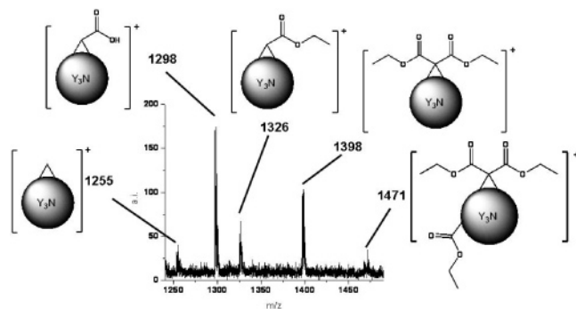
Figure 2. MALDI spectrum of a sample of 1 , Y_3N@C_{80}-C(CO_2Et)_2 , after chemical reduction with sodium metal in THF. No traces of the pristine Y_3N@C_{80} were detected (see Supporting Information).
