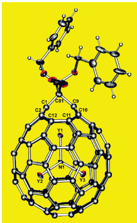
Figure 3. A drawing of the Bingel adduct Y_3N@C_{80}-C(CO_2CH_2Ph)_2 with 50% thermal contours for those atoms refined anisotropically and uniform circles for the carbon atoms of the fullerene. Only one orientation of the fullerene cage is shown, and only the major orientation of the Y_3N group is shown. Interatomic distances: Y1–N, 2.066(8); Y2–N, 2.042(9); Y3–N, 2.098(9) Å.
