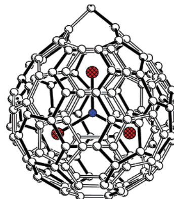
Figure 4. A drawing showing the two orientations of the fullerene cage and the major (0.70 occupancy) orientation of the Y_3N unit in the Bingel adduct Y_3N@C_{80}-C(CO_2CH_2Ph)_2 .
