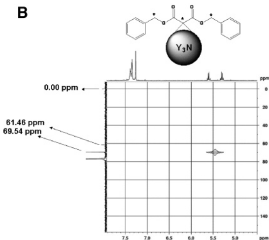
Figure 7. (A) ^{13}\text{C} NMR spectra of ^{13}\text{C} -labeled bis(benzyloxycarbonyl) bromomalonate (top) and that of the adduct 2 , \text{Y}_3\text{N}@C_{80}-\text{C}(\text{CO}_2\text{CH}_2\text{Ph})_2 (bottom) in \text{CDCl}_3 . (B) HMQC spectrum of ^{13}\text{C} -labeled 2 , \text{Y}_3\text{N}@C_{80}-\text{C}(\text{CO}_2\text{CH}_2\text{Ph})_2 .
