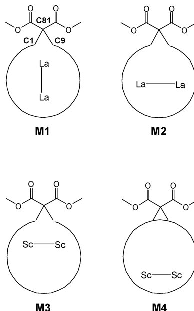
Scheme 2. Schematic Representations of Open and Closed Functionalized M 2 @C 80 Cages for Different Positions of the La 2 (Models M1 and M2 ) and Sc 2 (Models M3 and M4 ) Encapsulated Units
